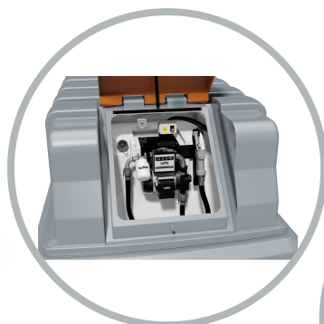
External pump
